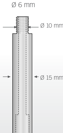
Ø 10 mm LS-237 90 mm
