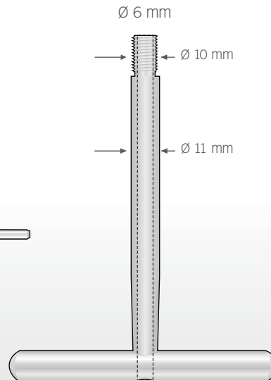
Ø 6 mm LS-238 130 mm
